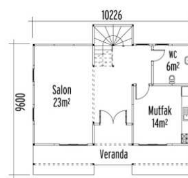
67 m 2 (67m 2 + 21m 2 ) ZEMİN KAT PLANI
