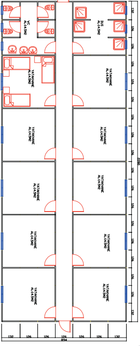
Yatakhane 136 m 2
